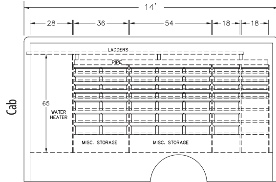
Driver's Side 14'
