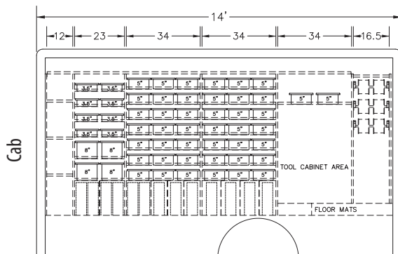
Driver's Side
