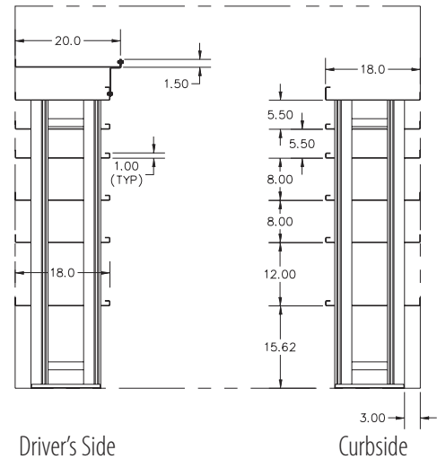
SECTION VIEW
