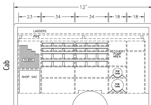
Driver's Side
