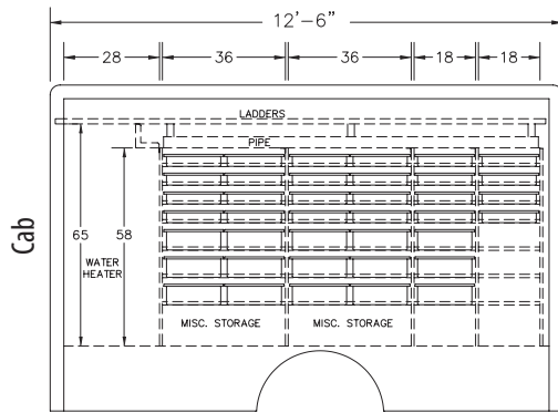
Driver's Side 12'
